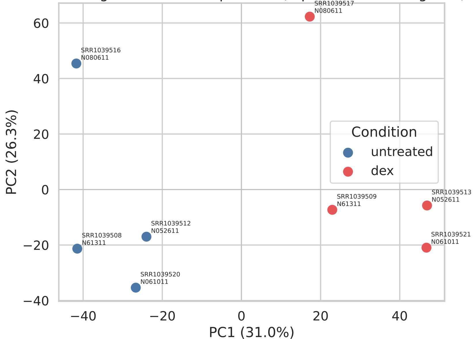
PCA of log2 normalized expression (top 5,000 variable genes)
