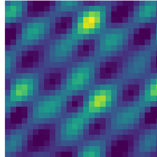
2-body Appx.
