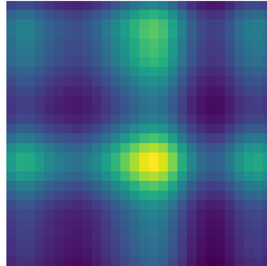
1-body Appx.
