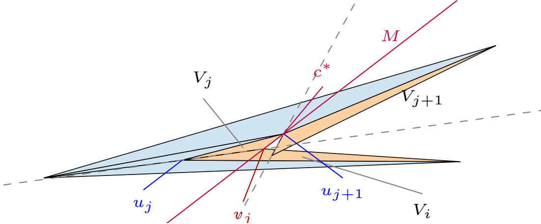
Figure 2: A thin above-base overlap (no hypothesis): the dashed cut-edge lines, the point c^* and the line M of §3. Here \nu_i + \nu_j > \pi and V_i crosses M .
