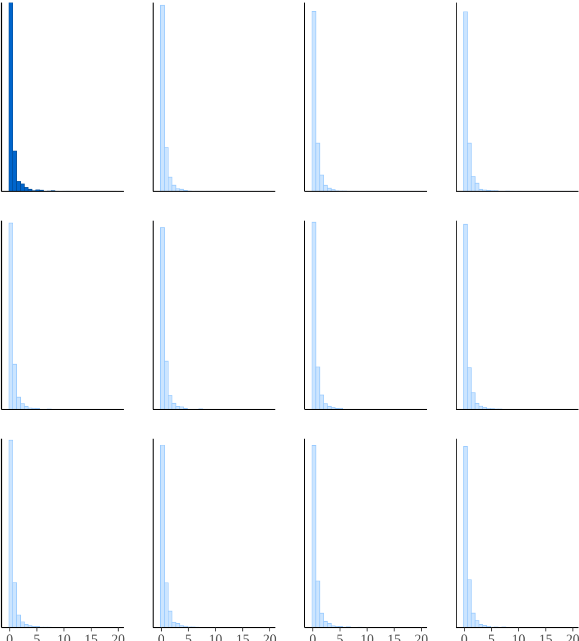
AMRO
