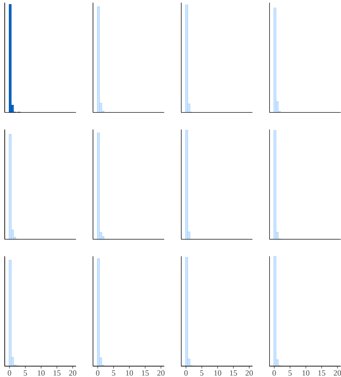
ACFL
