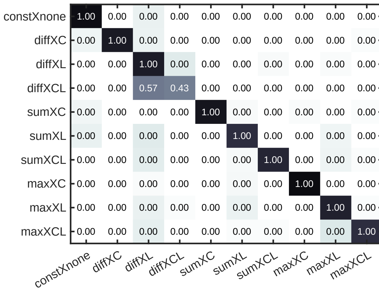
Fit model
