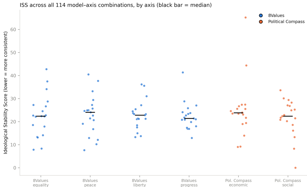
Figure 3: Ideological Stability Score for all 114 model-axis combinations, grouped by axis. Each point is one model; the black bar marks the axis median.
