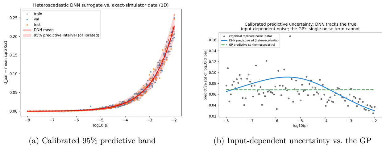
Figure 1: One-dimensional surrogate calibration. Left: the calibrated 95% predictive band tracks the response curve across the full range of \theta . Right: the network’s heteroscedastic predictive standard deviation (which enters the ABC acceptance kernel directly) tracks the true input-dependent replicate noise, while the GP’s single homoscedastic noise term is flat by construction.
