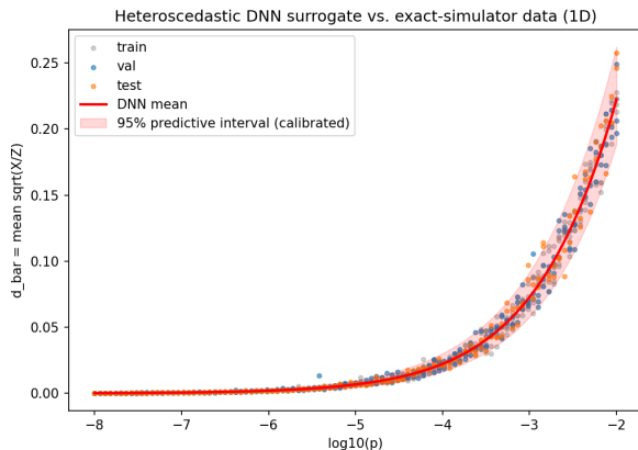
(a) Calibrated 95% predictive band
