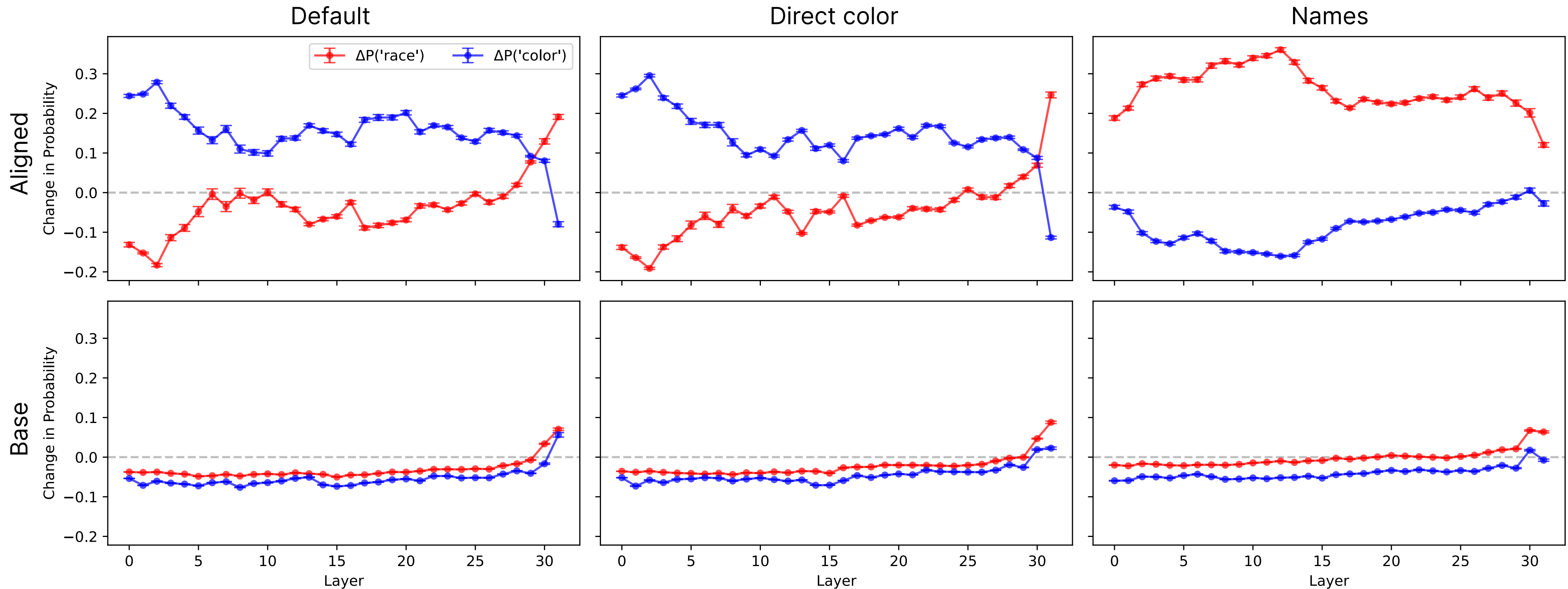
(b) Activation patching probability shifts
