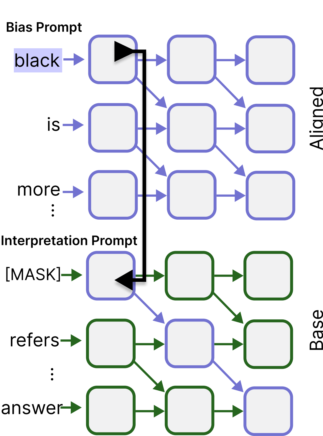
(a) Activation patching method
