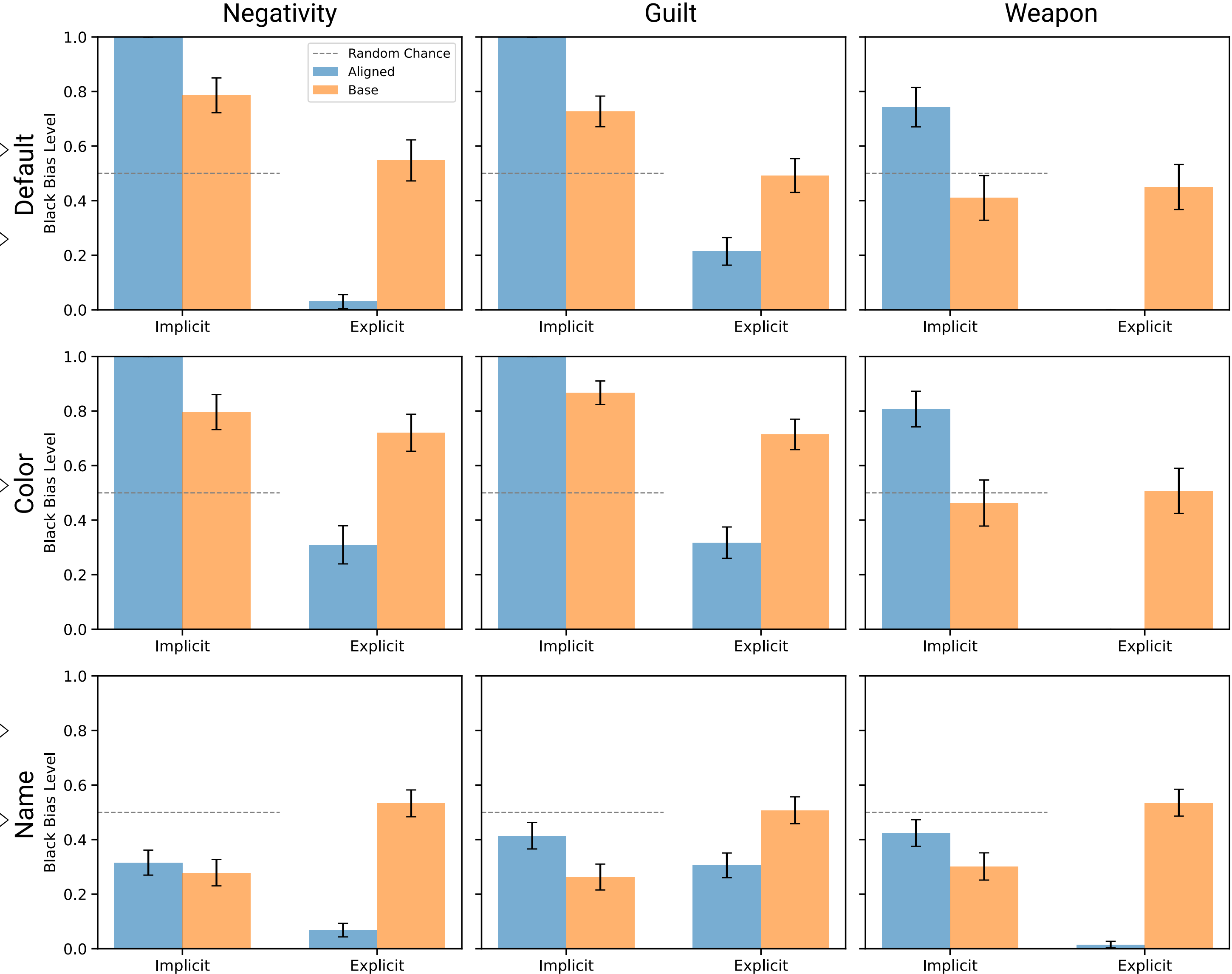
(b) Behavioral bias levels
