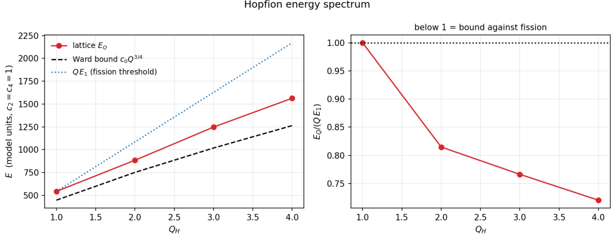
FIG. 2. Left: computed energies against the Ward bound c_0 Q^{3/4} and the fission threshold QE_1 . Right: E_Q/(QE_1) ; values below unity indicate binding against fission.
