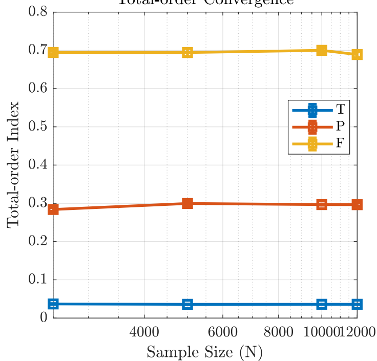
Total-order Convergence
