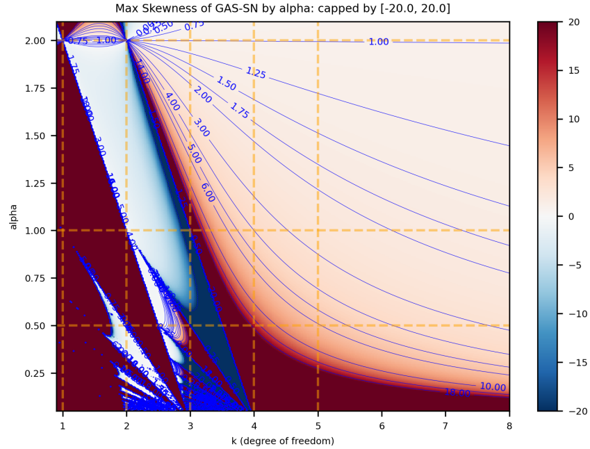
FIGURE 12.4. The contour plot of skewness of the half-GSaS L_{\alpha,k}^+ by (k, \alpha) . This represents the maximum skewness that the GAS-SN family can achieve.
