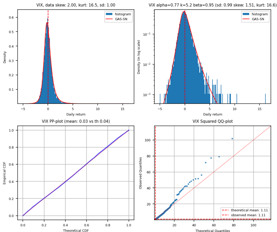
FIGURE 12.6. MLE fit of daily VIX returns from 1990 to mid-2025. The data are standardized to unit variance. Sample skewness is 2.0, and sample kurtosis is 16.5. \hat{\Theta} = \{\alpha = 0.77, k = 5.2, \beta = 0.95\} . Top left: density and histogram. Top right: log-density and histogram. Bottom left: PP-plot. Bottom right: QQ-plot of the quadratic form.
