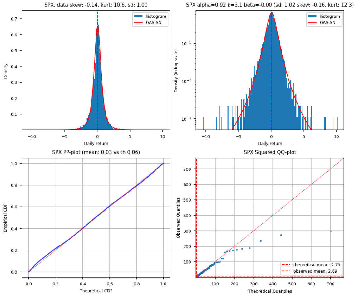
FIGURE 12.7. MLE fit of daily SPX log returns from 1990 to mid-2025. The data are standardized to unit variance. Sample skewness is -0.14 , and sample kurtosis is 10.6 . \hat{\Theta} = \{\alpha = 0.92, k = 3.1, \beta = 0.0\} . Top left: density and histogram. Top right: log-density and histogram. Bottom left: PP-plot. Bottom right: QQ-plot of the quadratic form.
