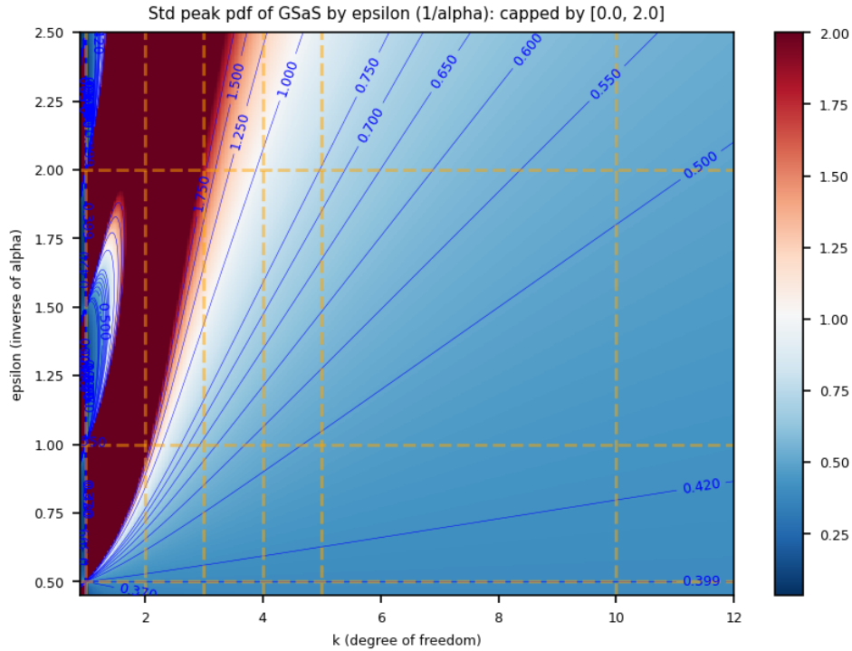
FIGURE 12.3. The contour plot of standardized peak density in GSaS by (k, \epsilon) , where \epsilon = 1/\alpha .
