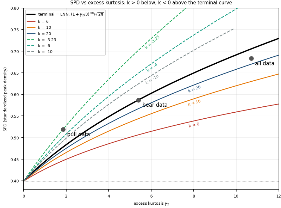
FIGURE 12.4. The relation between excess kurtosis \gamma_2 and the standardized peak density (SPD) in GSaS, indicated by representative k 's. We added three points from the SPX global regime analysis to illustrate the usage (see footnote). "All data" is the statistics from the full dataset. "Bull data" is the statistics from the bull state, which lies in the negative k branch. "Bear data" is the statistics from the bear state, which lies on the terminal curve.
