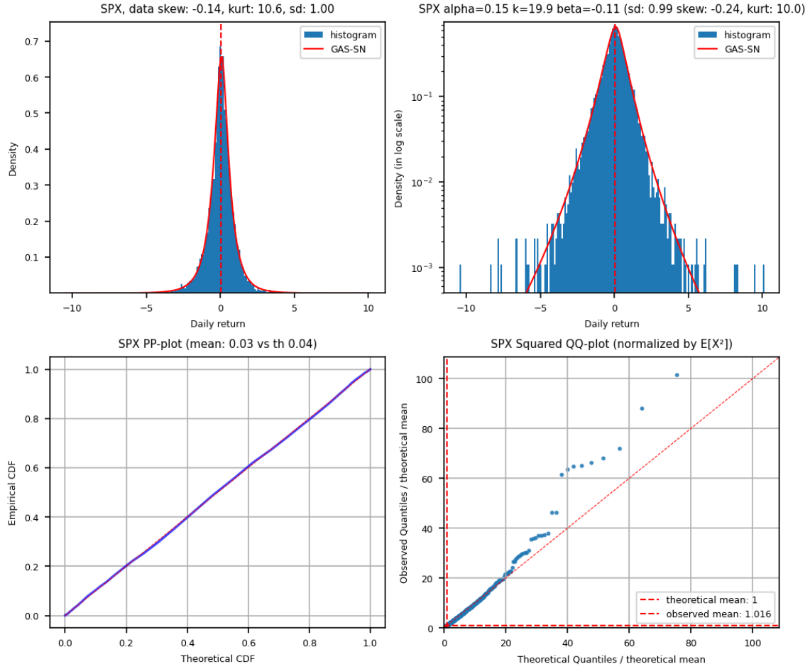
FIGURE 12.8. MLE fit of daily SPX log returns from 1990 to mid-2025. The data are standardized to unit variance. Sample skewness is -0.14 , and sample kurtosis is 10.6 . \hat{\Theta} = \{\alpha = 0.15, k = 19.9, \beta = -0.11\} . Top left: density and histogram. Top right: log-density and histogram. Bottom left: PP-plot. Bottom right: QQ-plot of the quadratic form.
