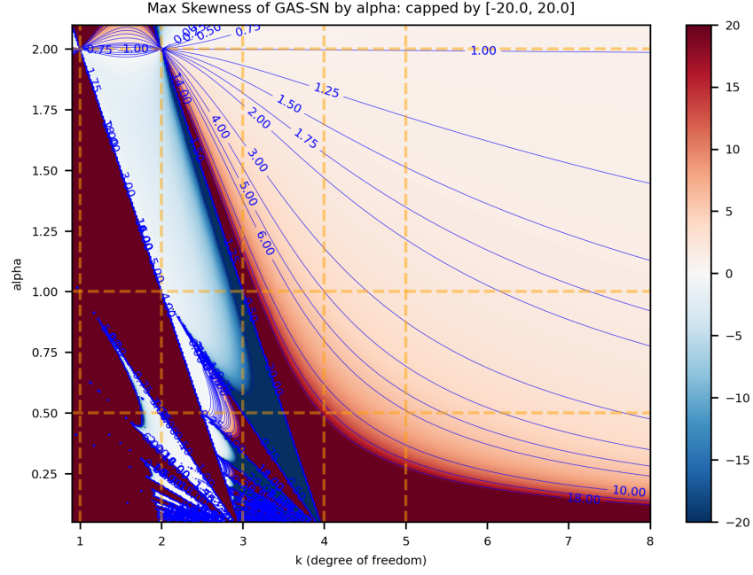
FIGURE 12.5. The contour plot of skewness of the half-GSaS L_{\alpha,k}^+ by (k, \alpha) . This represents the maximum skewness that the GAS-SN family can achieve.
