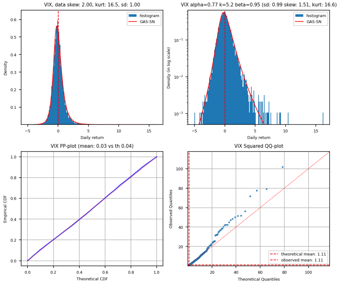
FIGURE 12.7. MLE fit of daily VIX returns from 1990 to mid-2025. The data are standardized to unit variance. Sample skewness is 2.0, and sample kurtosis is 16.5. \hat{\Theta} = \{\alpha = 0.77, k = 5.2, \beta = 0.95\} . Top left: density and histogram. Top right: log-density and histogram. Bottom left: PP-plot. Bottom right: QQ-plot of the quadratic form.
