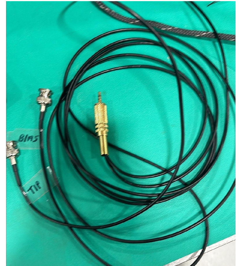
Custom TRS to 2 BNC Cable
