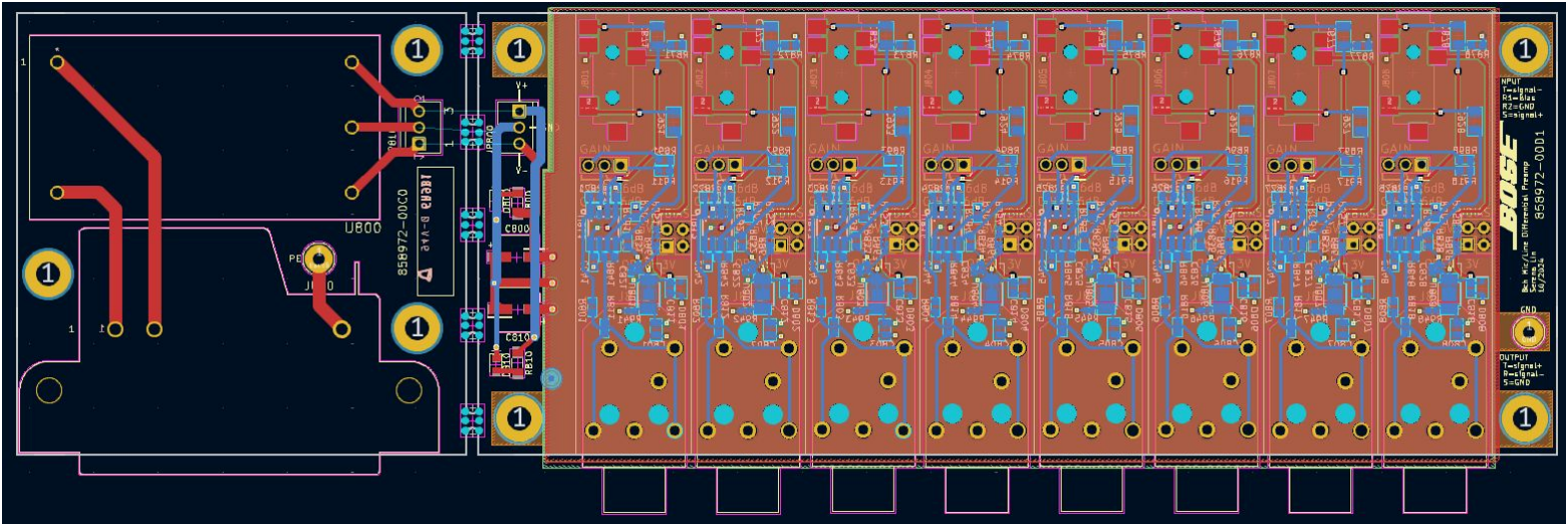
Layout View 8 Channels & Power Supply
