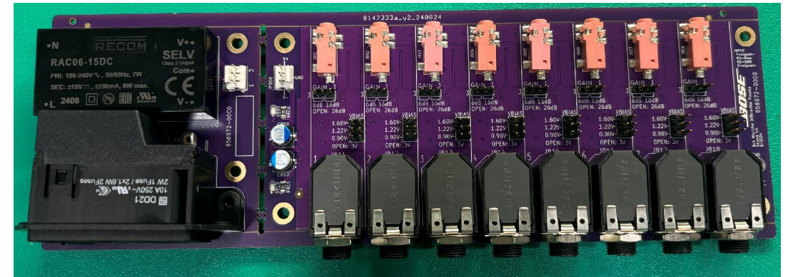
New Differential Pre-Amp Front View
