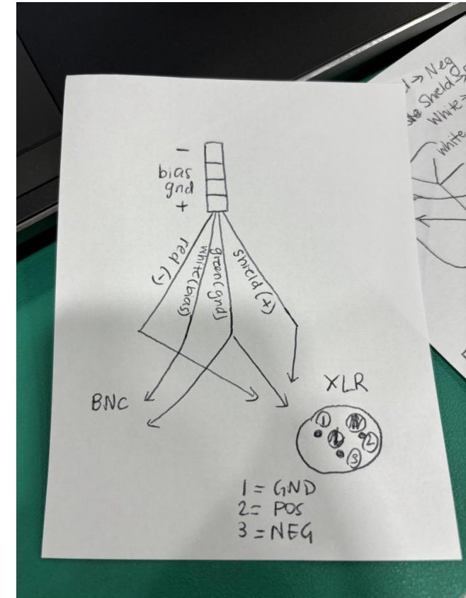
Schematic for Custom TRRS 1 BNC & 1XLR Cable
