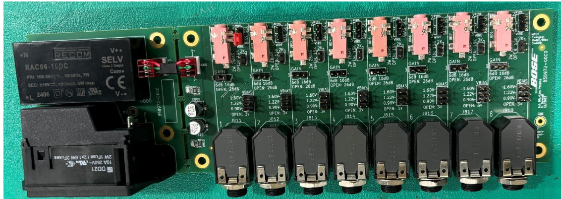
Single Ended Pre-Amp Front View
