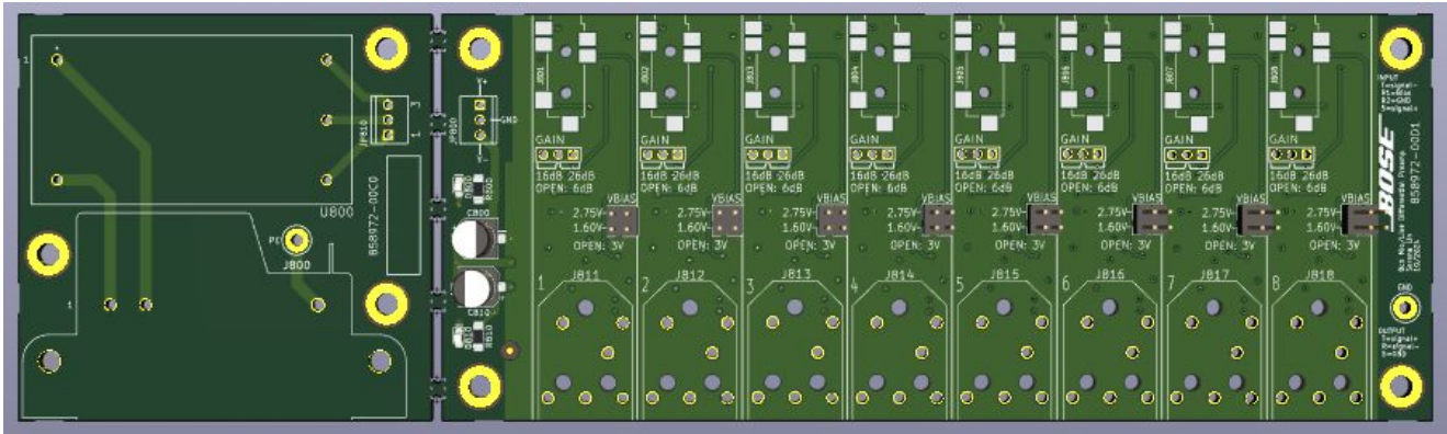
Ki Cad 3D Viewer
