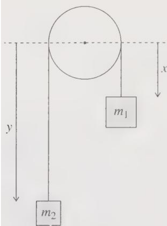
Figure 3 An Atwood machine consisting of two masses, m_1 and m_2 , suspended by a massless inextensible string that passes over a massless, frictionless pulley of radius R . Because the string's length is fixed, the position of the whole system can be specified by a single variable, which we can take to be the distance x .
