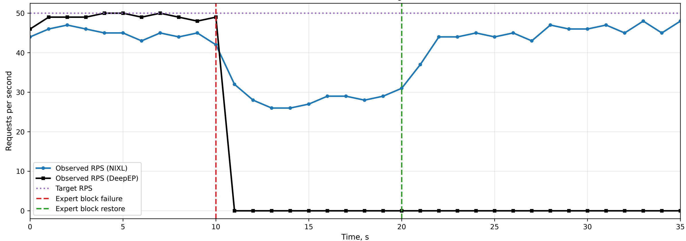
Fault tolerance benchmark, target 50 RPS
