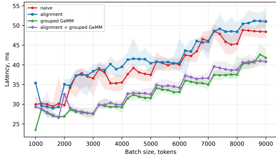
NIXL: High expert activation
