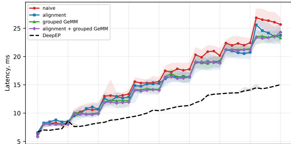
NIXL: Low expert activation
