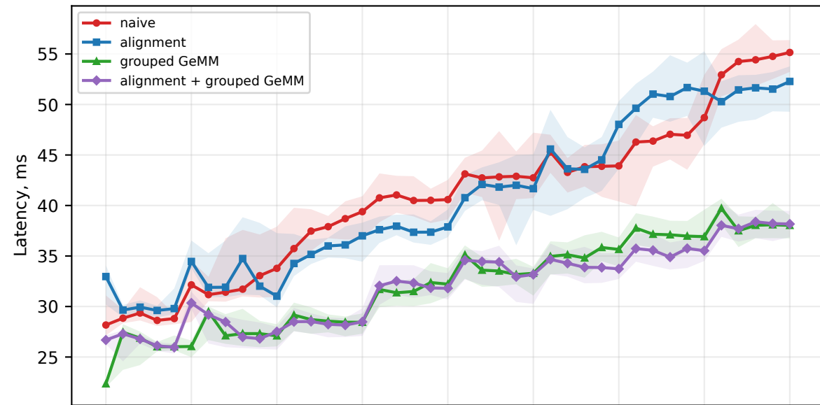
NIXL: High expert activation
