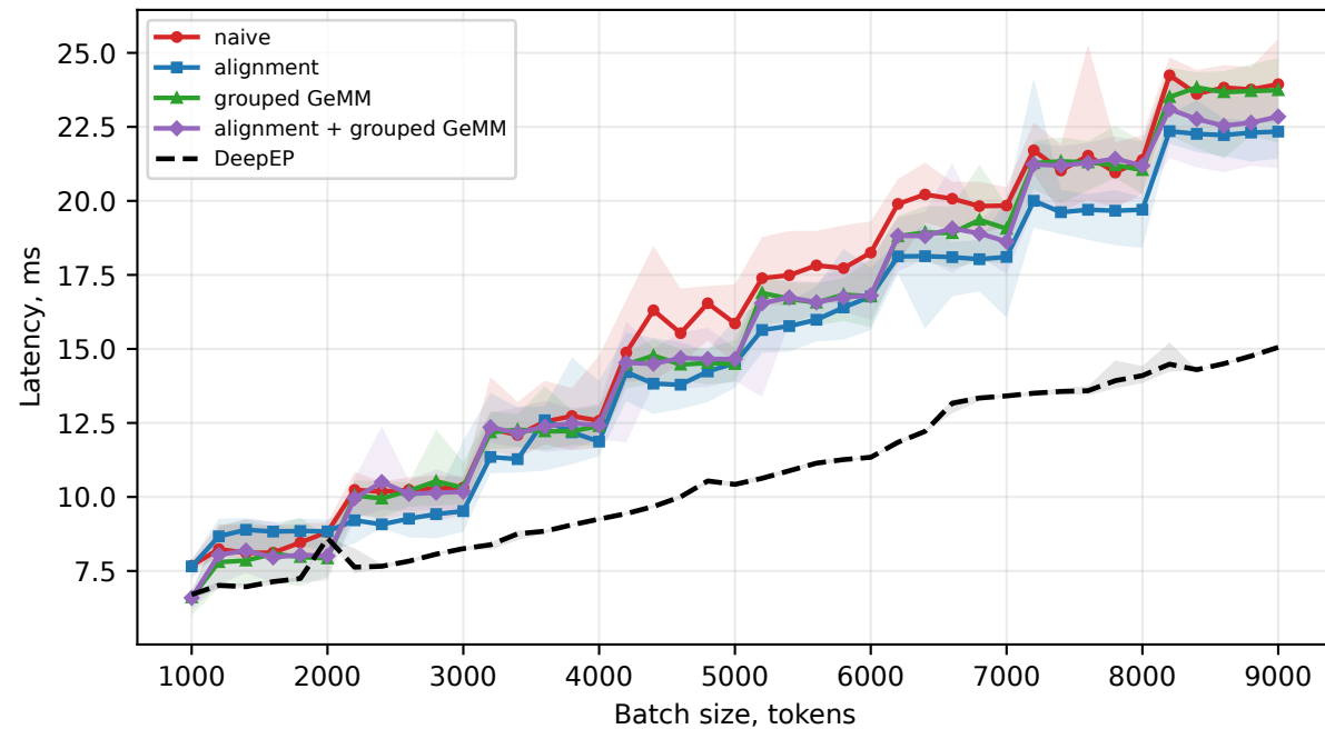
NIXL: Low expert activation
