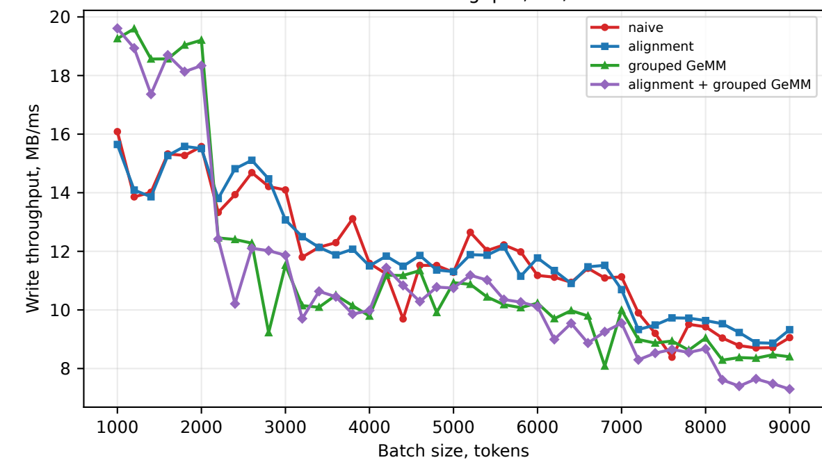
NIXL: Write throughput, MB/ms
