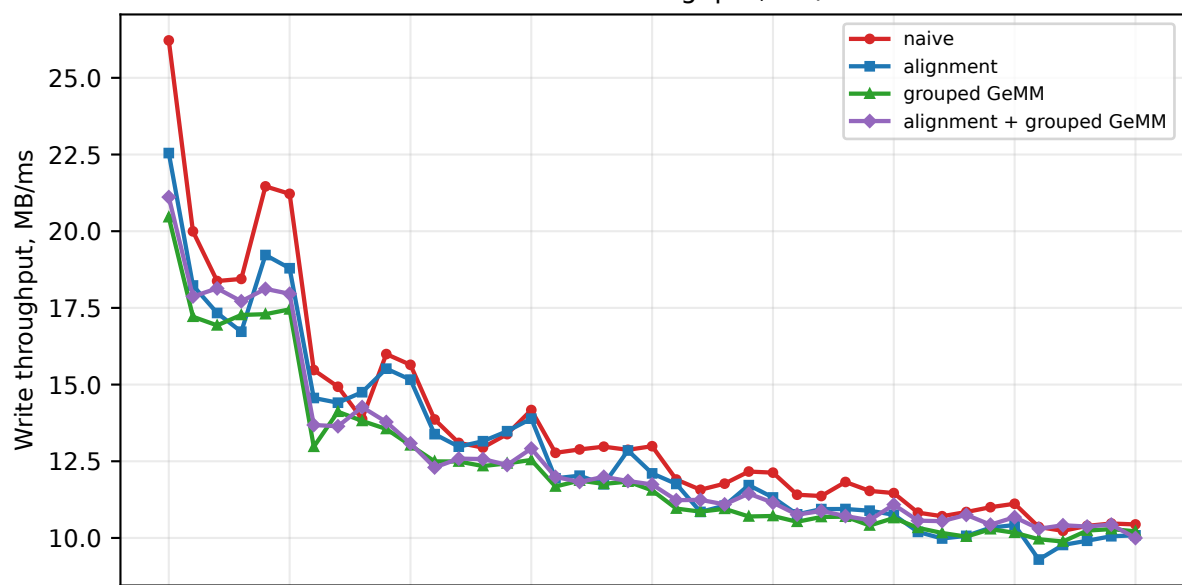
NIXL: Write throughput, MB/ms
