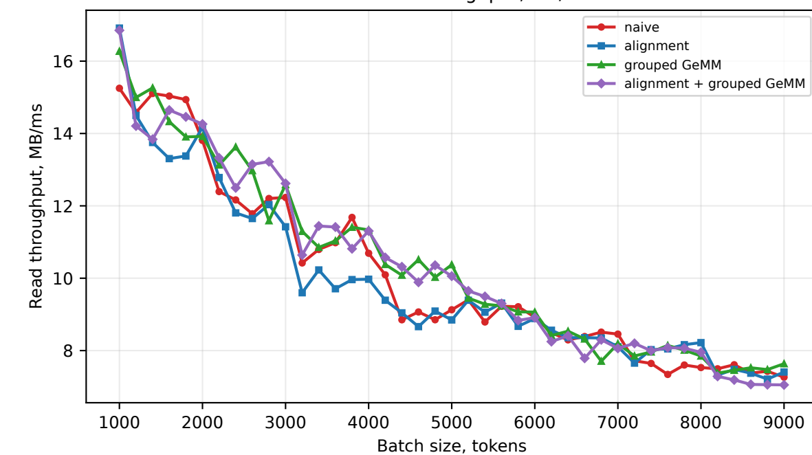
NIXL: Read throughput, MB/ms
