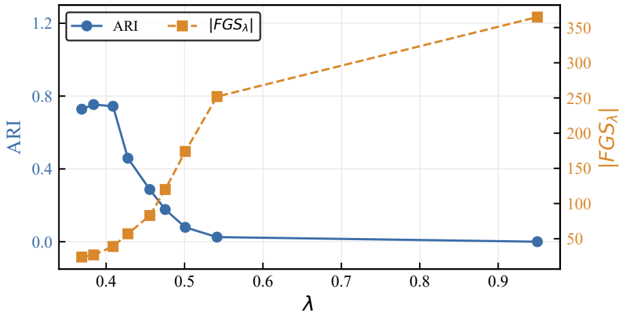
Layer-wise ARI and granule count (Dermatology)
