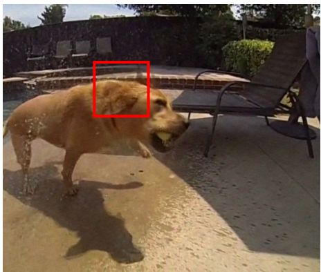
ComplexPhaseNet
