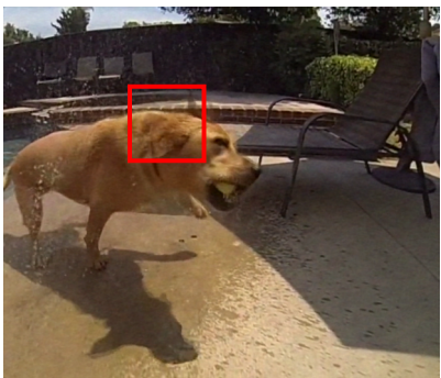
Easy Sample 115
