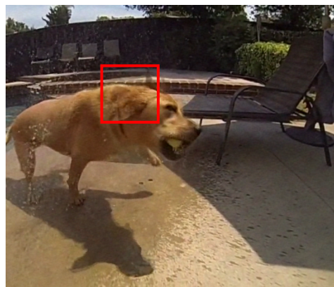
ComplexPhaseNet
