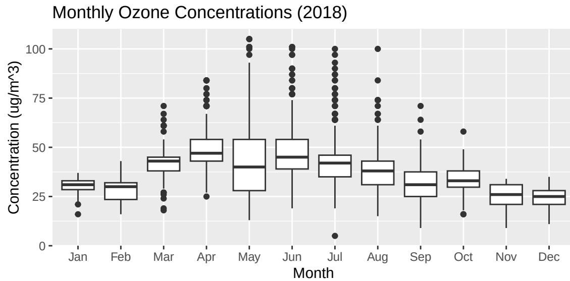
Figure 1: 2018 monthly ozone levels
