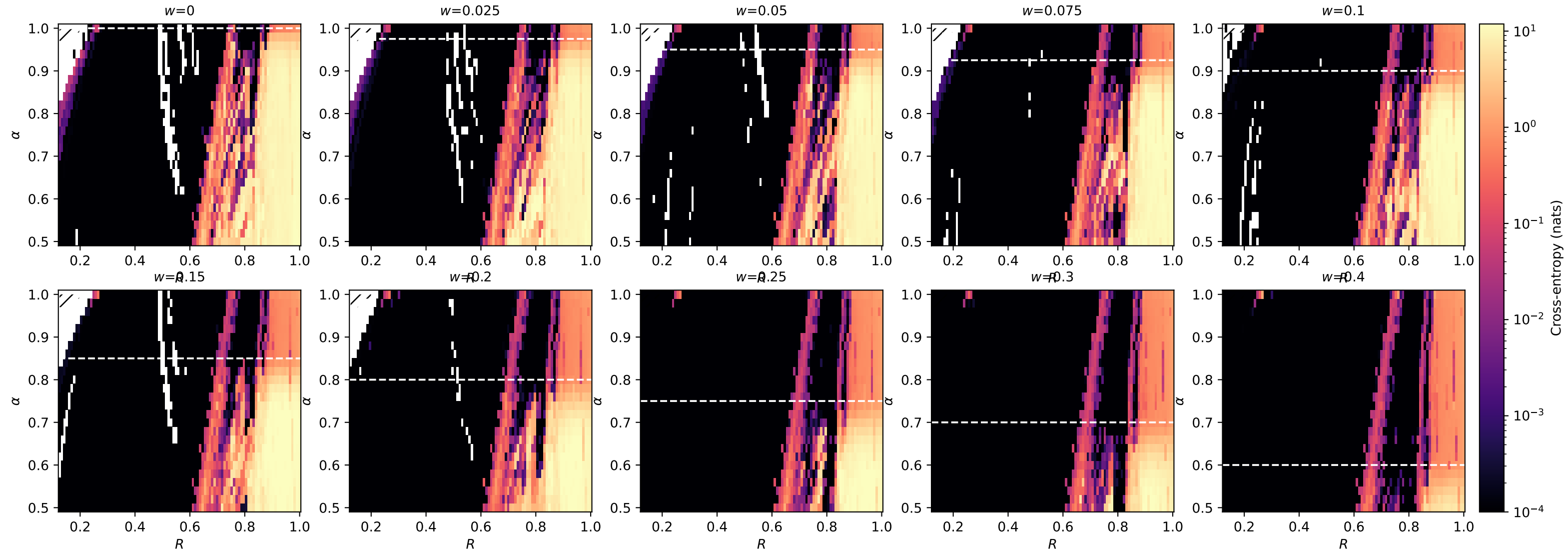
Cross-entropy over the (\alpha, R) plane. Dashed line: lower edge of the training band. Hatching: orbits die at the origin (trivially predictable).
