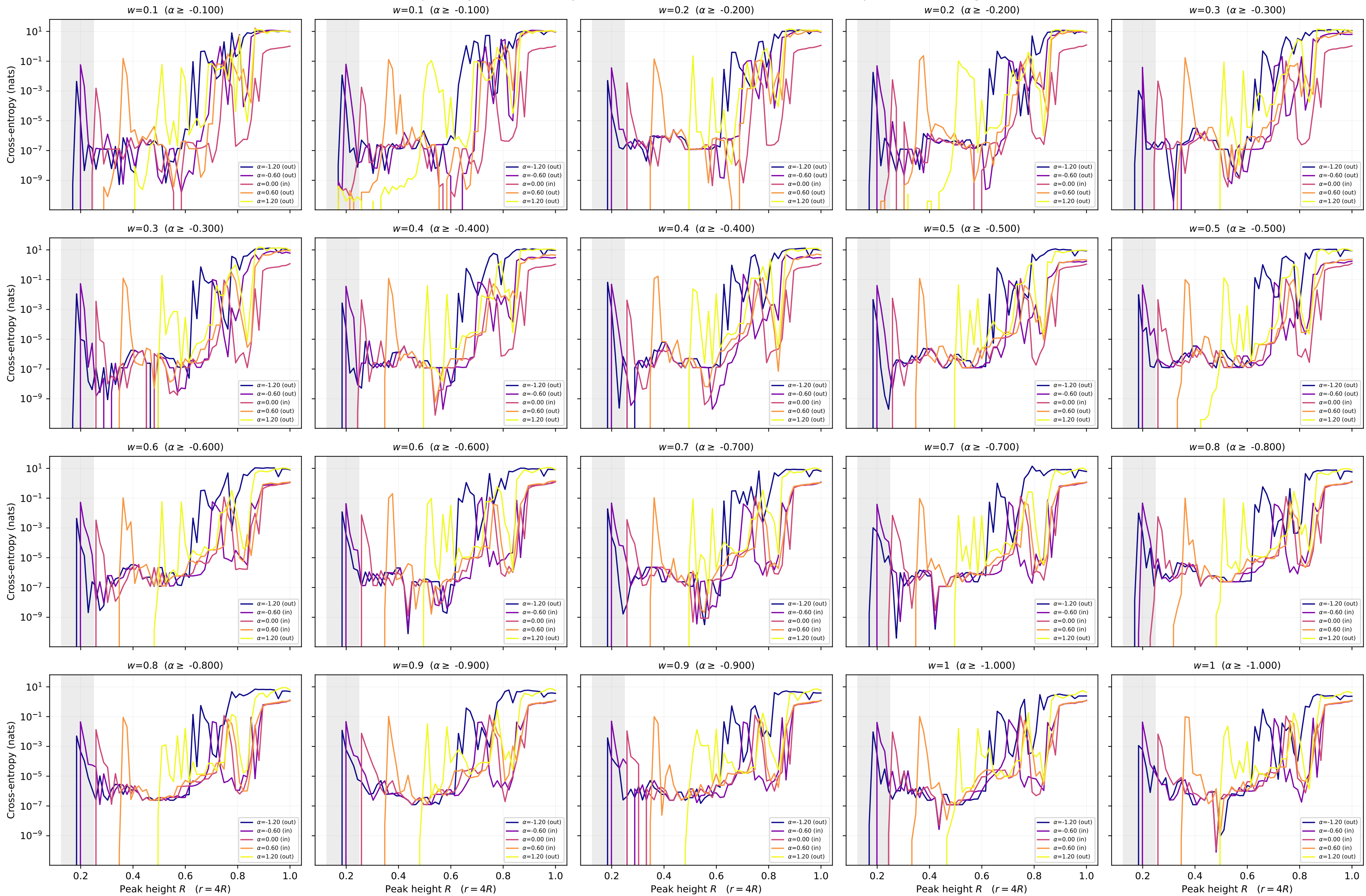
Loss vs peak height R at selected asymmetries; shaded band is R < 0.25 ( r < 1 ), where every orbit dies at the origin
