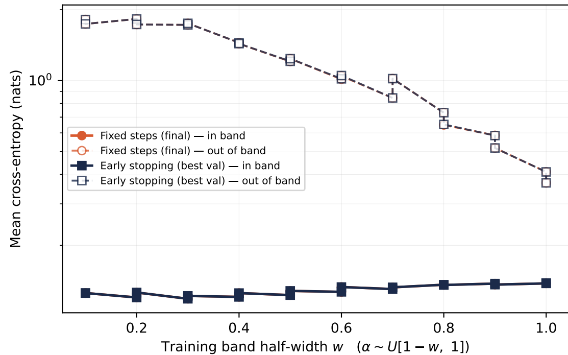
Generalization across \alpha ( w = 0 is train-on-logistic, zero-shot)
