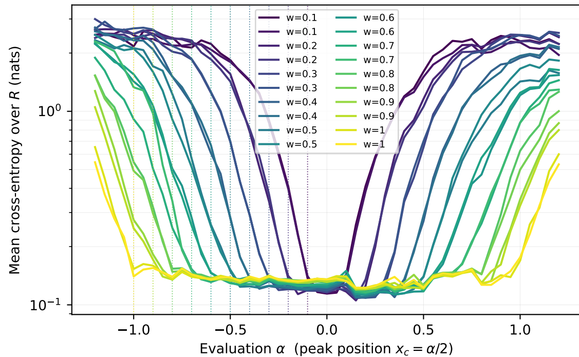
Loss vs asymmetry; dotted lines mark each band edge
