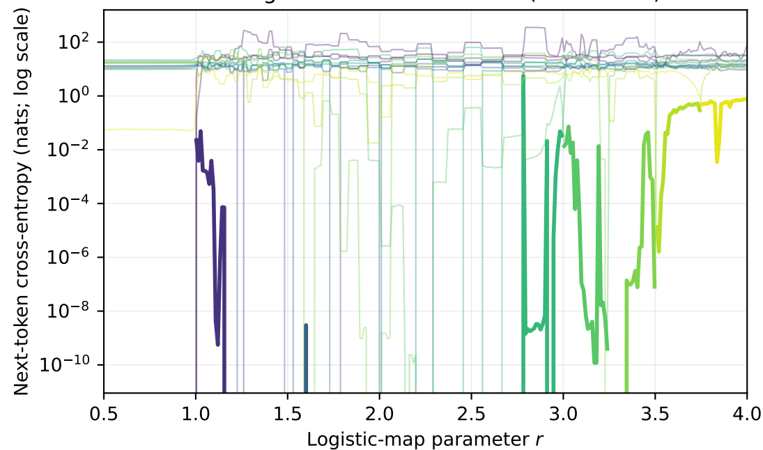
Training-window width = 0.25 (14 models)
