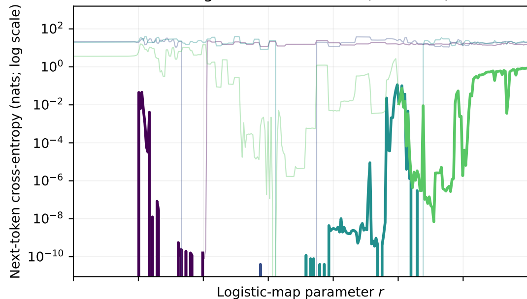
Training-window width = 0.25 (14 models)
