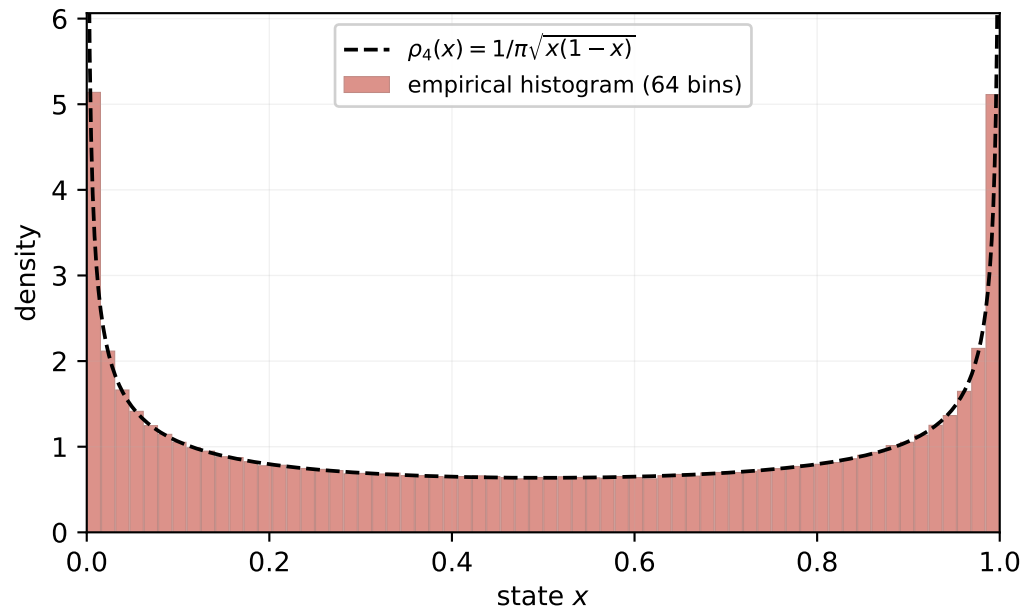
(c) Invariant measure, r = 4
