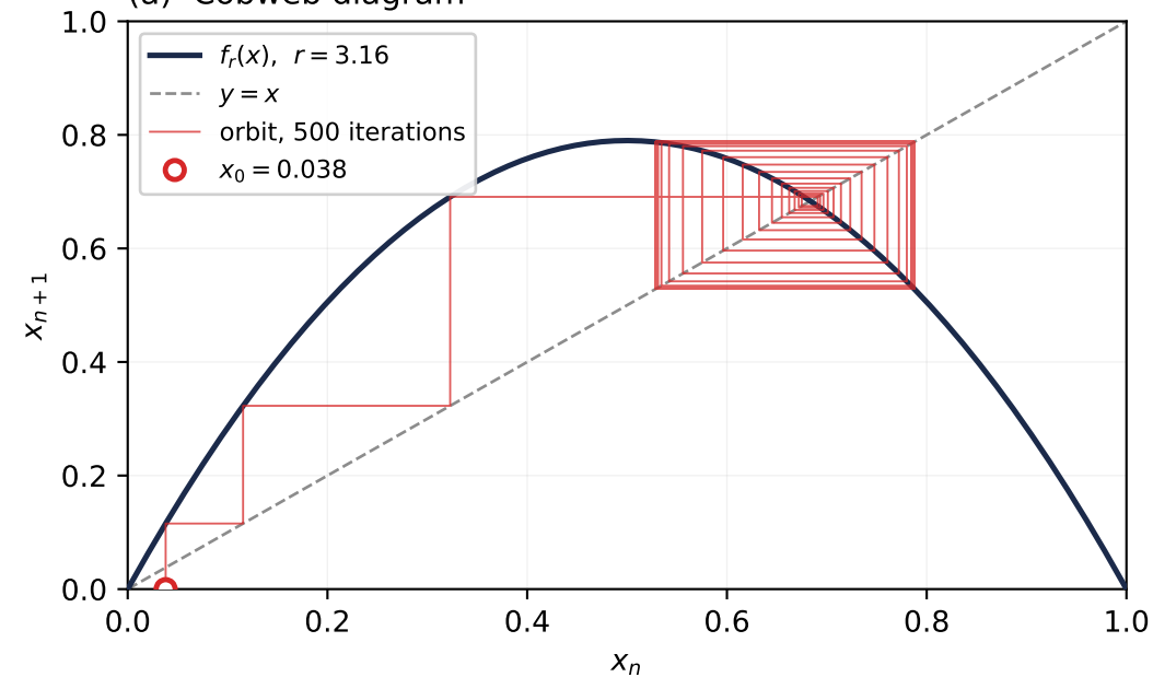
(a) Cobweb diagram
