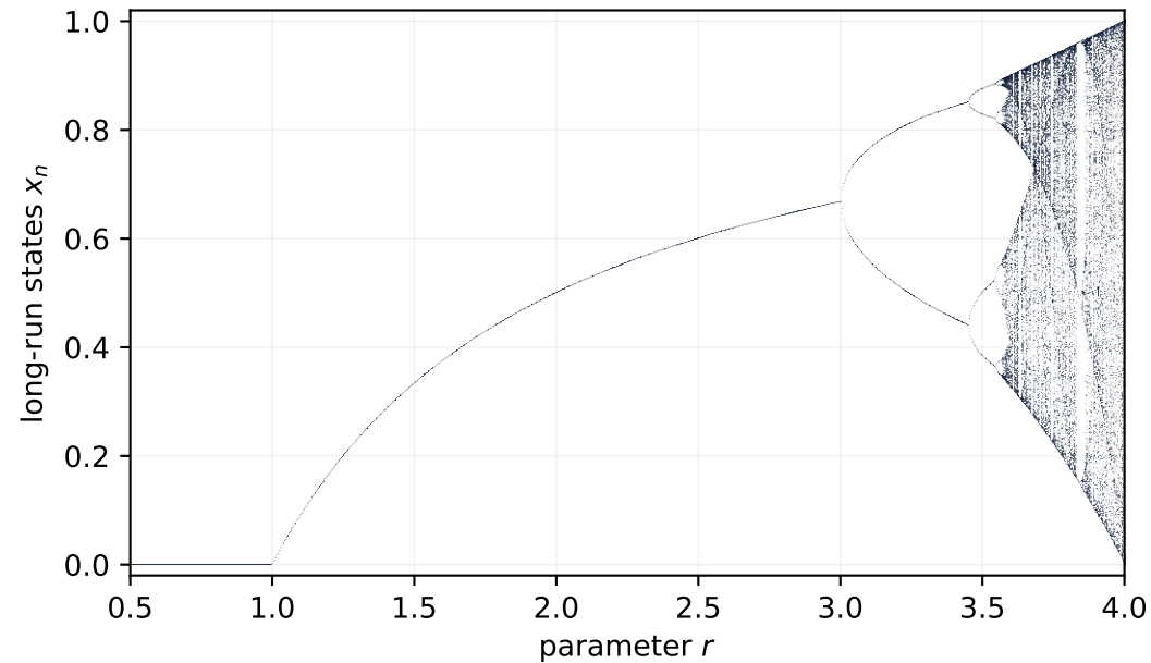
(b) Bifurcation diagram
