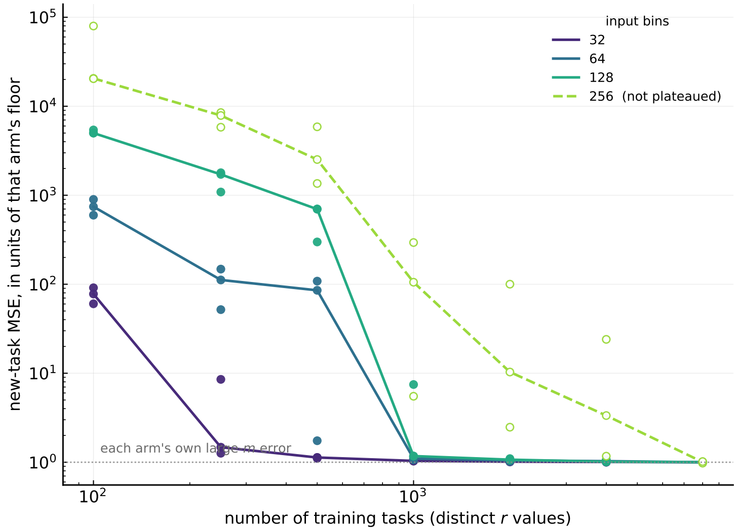
640k steps, square loss; every seed plotted, line is the median. Normalising by each arm's floor removes the 140x spread in where the curves end, so only the location of the drop distinguishes them. Points inside the transition: 0 of 7 at 32 bins, 2 at 64, 2 at 128, 4 at 256 — the grid is too coarse to place the threshold.
