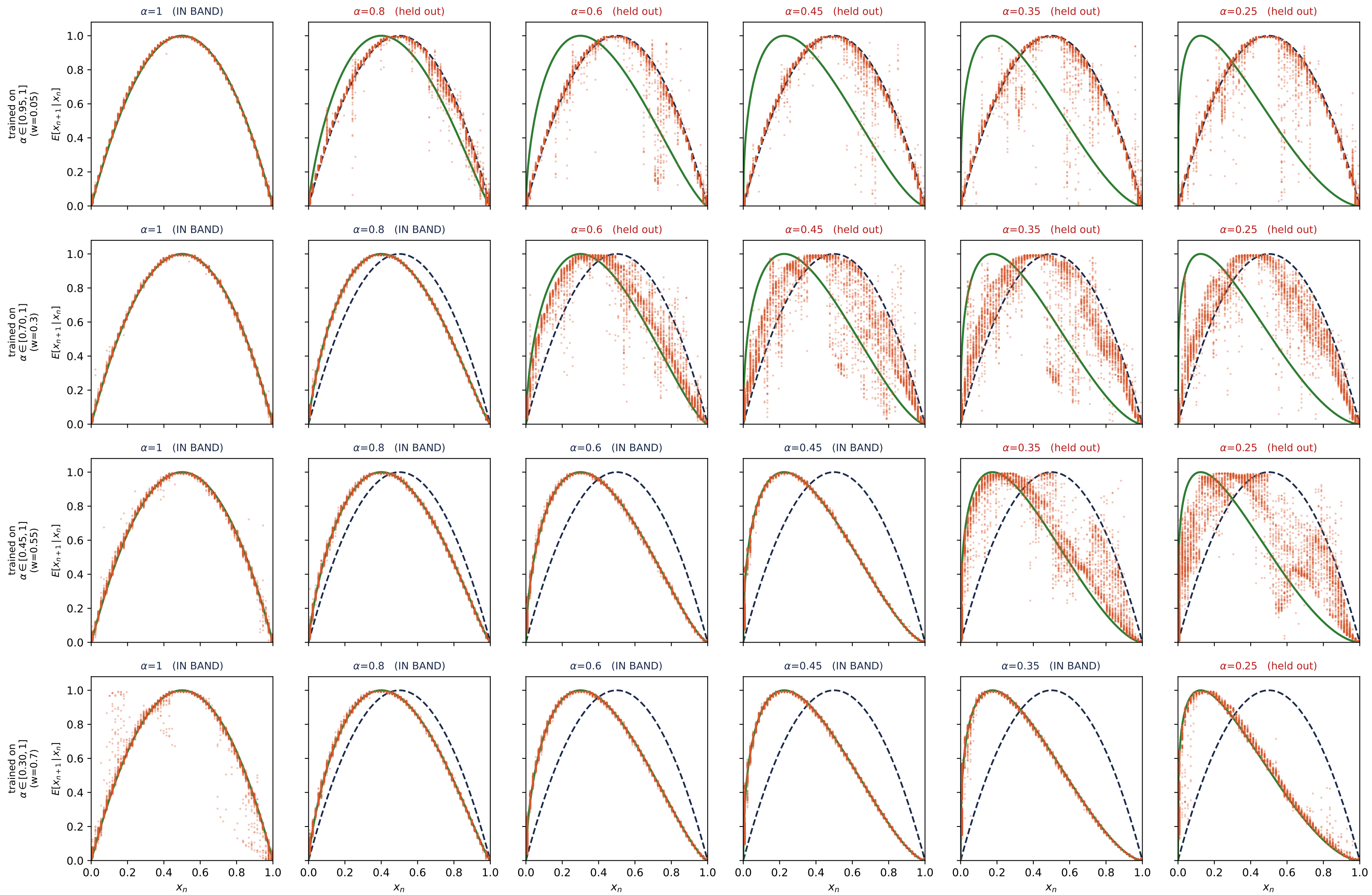
Implied return map at R = 1 : does the model track the true map, or the one it was trained on? Orange on green = it identified the map from context; orange on dashed navy = it is applying a memorized map
