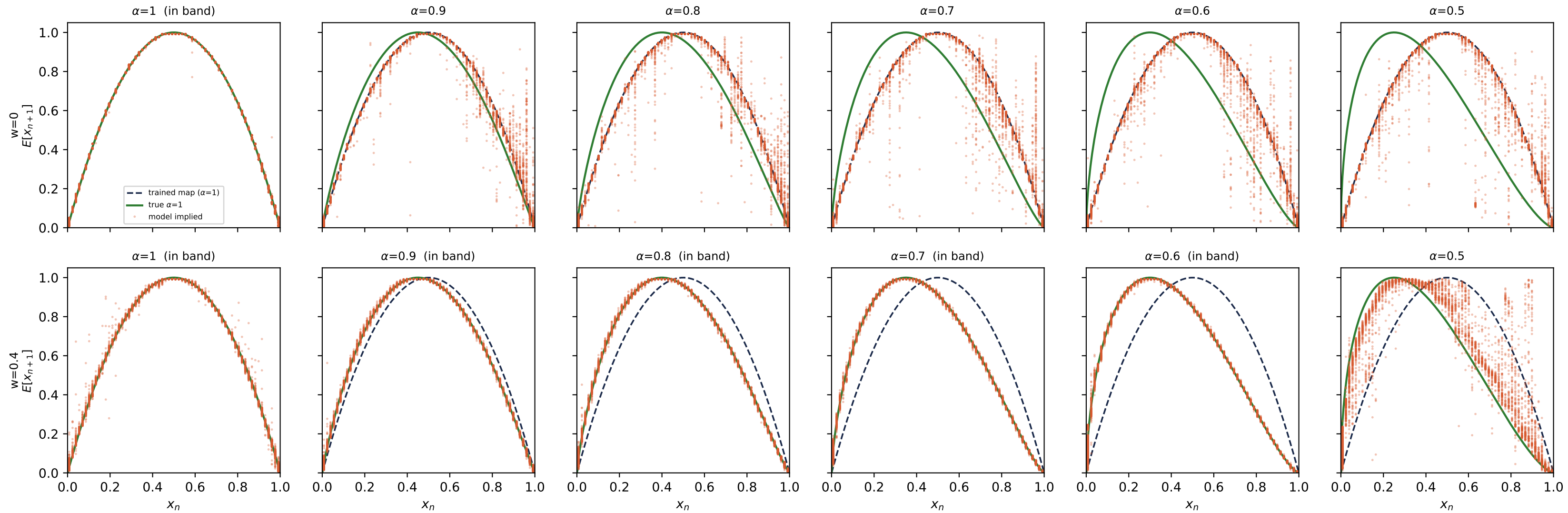
Implied return map at R = 1 : does the model track the true map or the one it was trained on?
