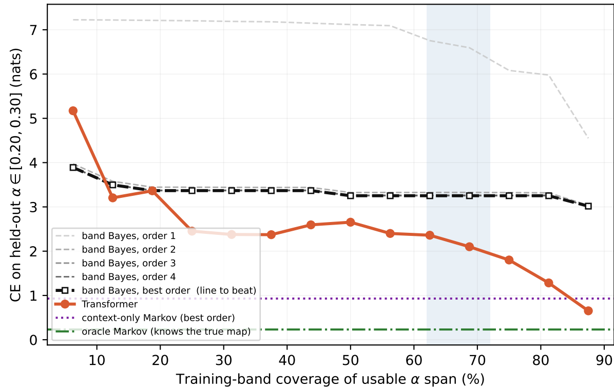
Held-out loss vs task diversity
