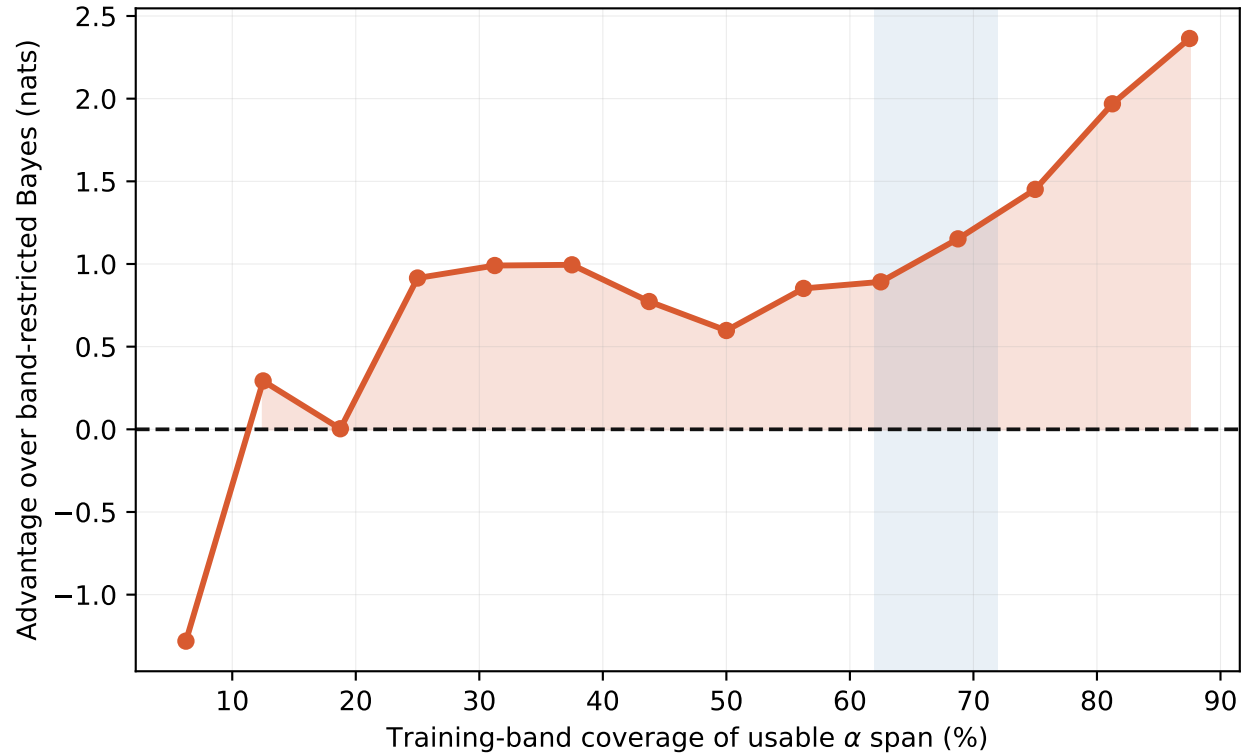
Generalization the pretraining distribution does not license (shaded band: predicted transition)
