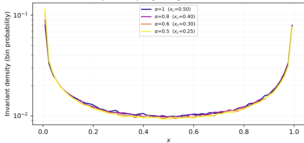
1-point occupancy: nearly identical across \alpha
