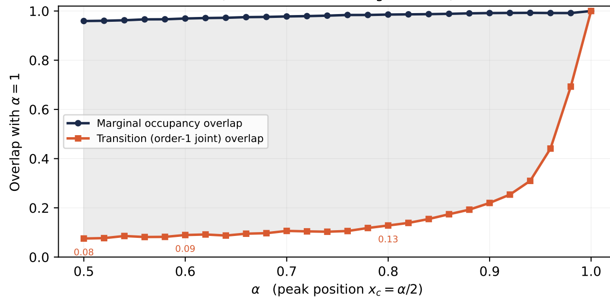
The two statistics disagree sharply (shaded: what the marginal hides)
