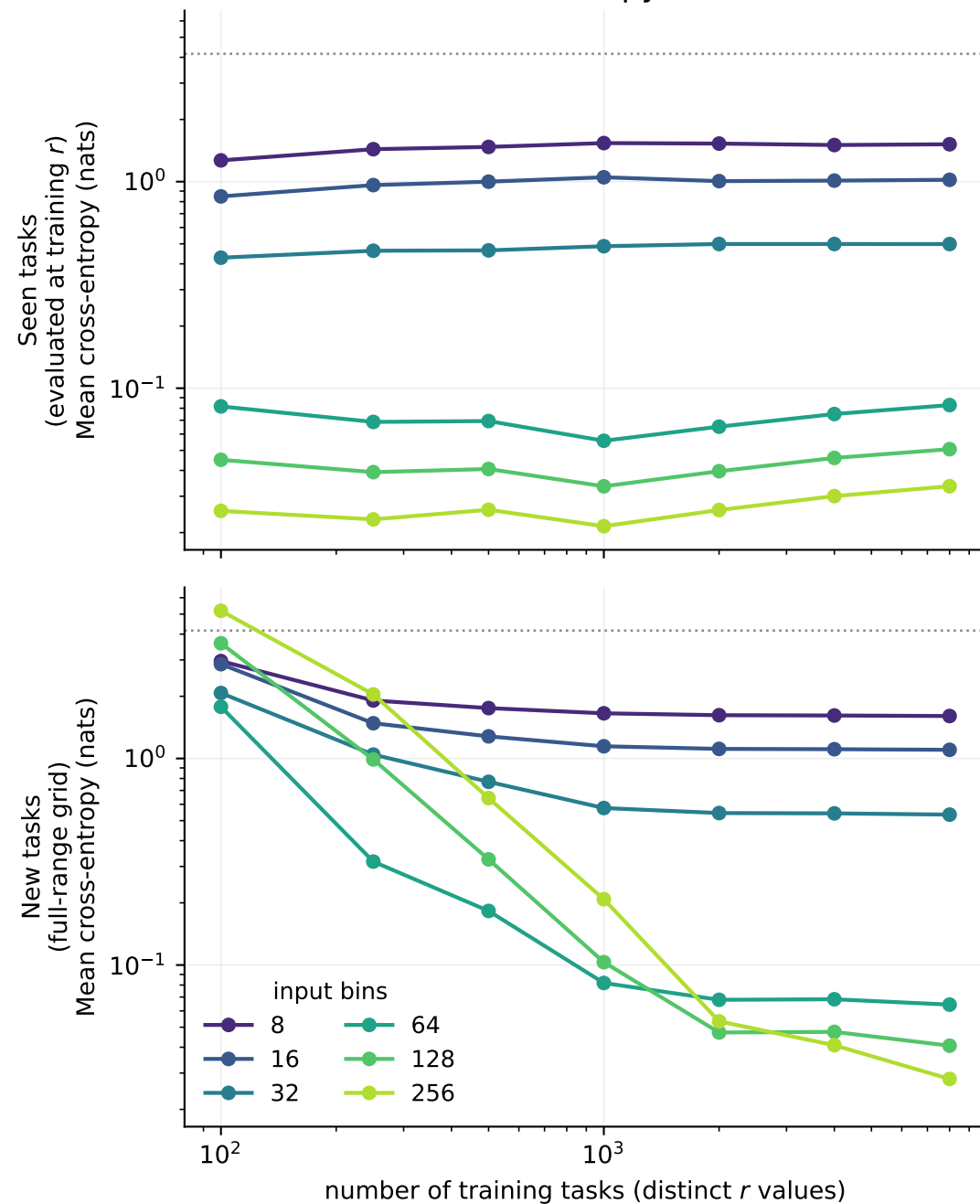
Cross-entropy loss
