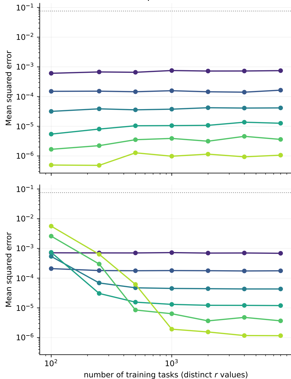
Square loss
