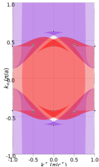
B3u
