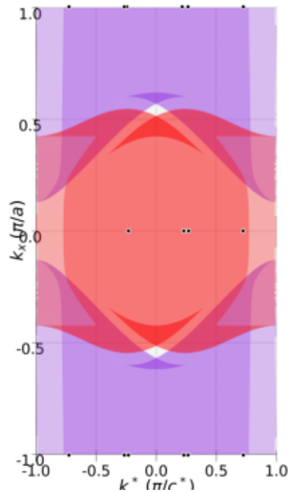
B2u
