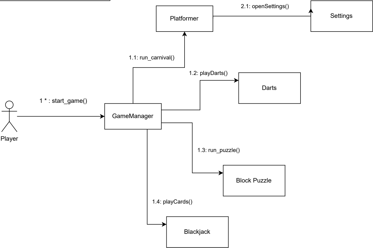
Communication Diagram Play Game
