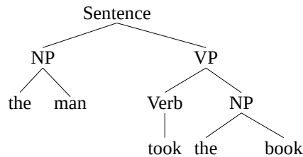
The first context-free grammar parse tree (Chomsky, 1956)
