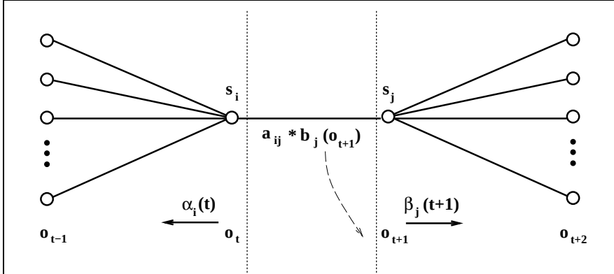
Figure D.3 Computation of the joint probability of being in state i at time t and state j at time t + 1 . The figure shows the various probabilities that need to be combined to produce P(q_t = i, q_{t+1} = j, O|\lambda) : the \alpha and \beta probabilities, the transition probability a_{ij} and the observation probability b_j(o_{t+1}) . After Rabiner (1989).
