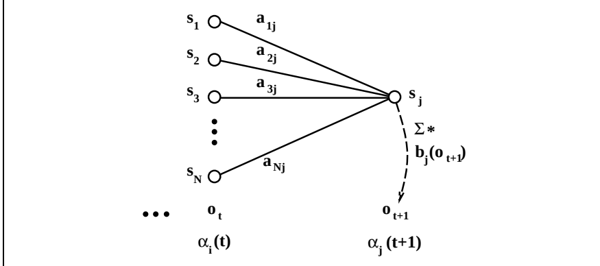
Figure D.1 The computation of \alpha_i(t) by summing all the previous values \alpha_{t-1} weighted by their transition probabilities a and multiplying by the observation probability b_i(o_{t+1}) . Of course in any given HMM many or most of the transition probabilities will be 0, so not all previous states will contribute to the forward probability of the current state.
