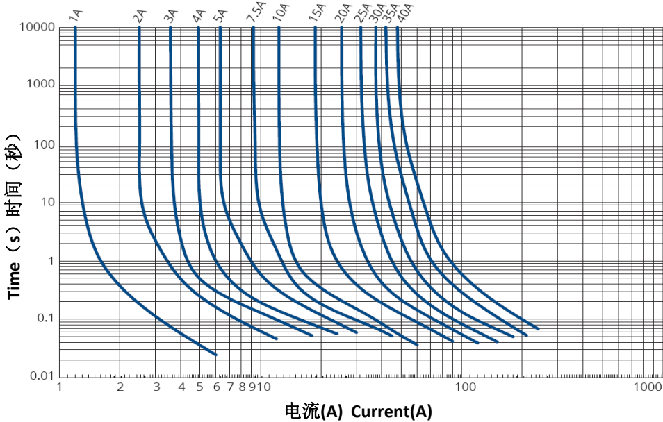
电流时间曲线图 Time-Current Characteristics
