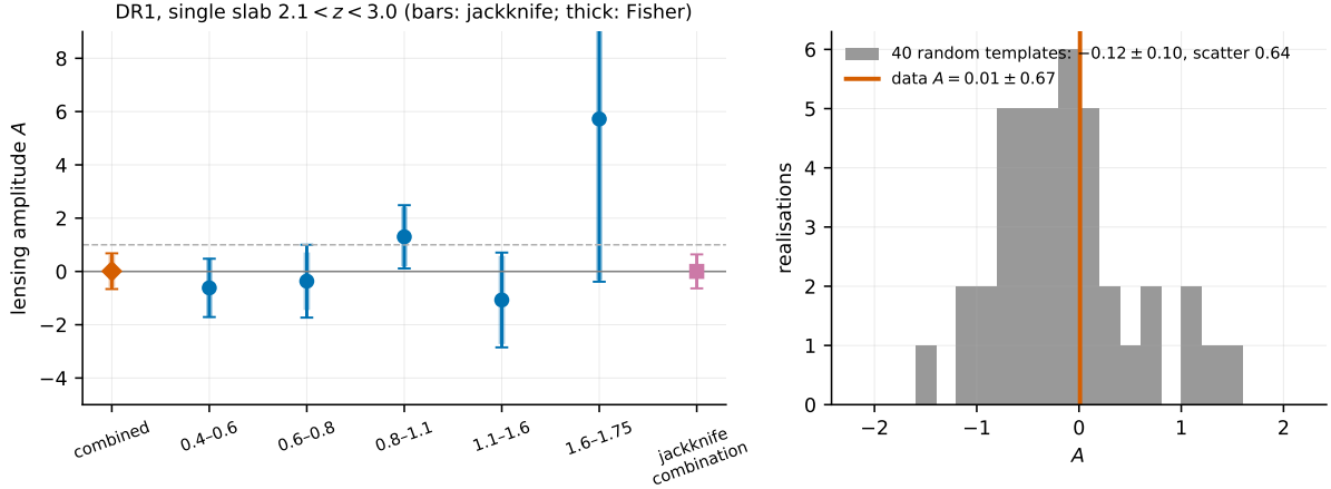
Figure 8: Left: the DR1 amplitudes per slice and combined (thin bars: jackknife, thick: Fisher) and the jackknife-covariance combination of the slices; the dashed line is the \Lambda CDM value. Right: the forty random-template amplitudes with the data value.
