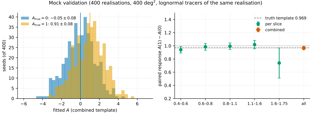
Figure 7: Mock validation on 400 realisations. Left: the combined-template amplitude for an unlensed ( A_{\text{true}} = 0 ) and a lensed ( A_{\text{true}} = 1 ) forest of the same realisations. Right: the paired response A(1) - A(0) per slice and combined, against the truth template.
