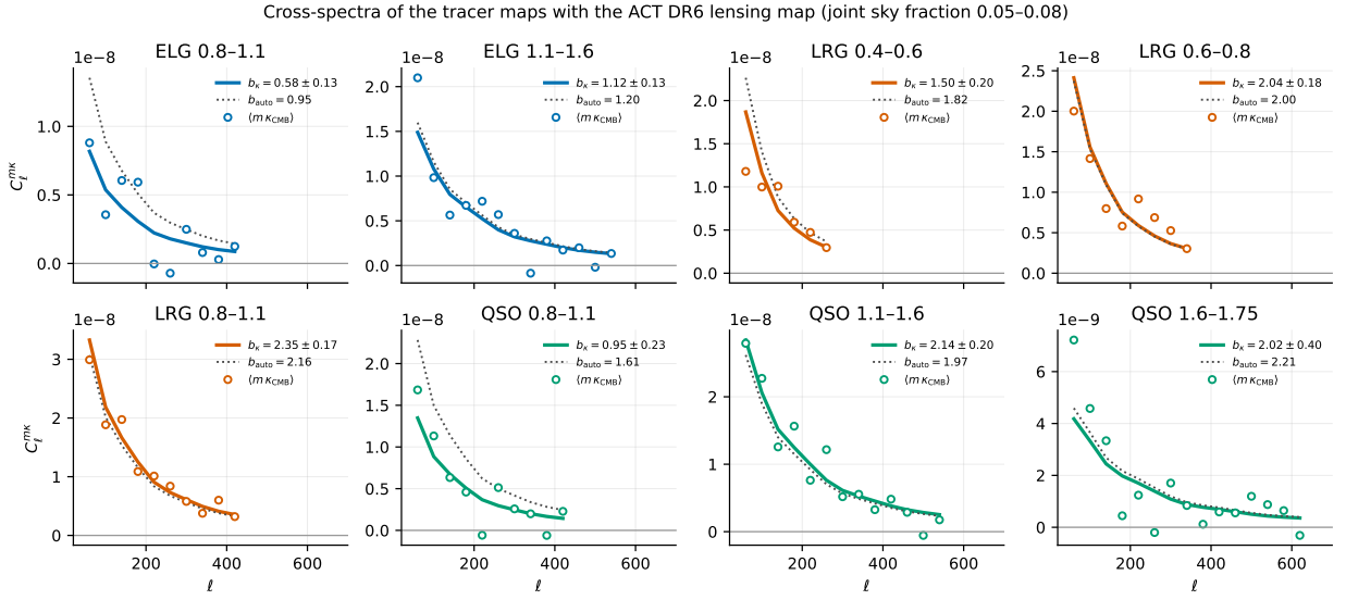
Figure 5: Cross-spectra of the unit-bias tracer maps with the ACT DR6 lensing map (points) with the theory scaled by the cross-correlation bias (solid) and by the auto-spectrum bias (dotted).
