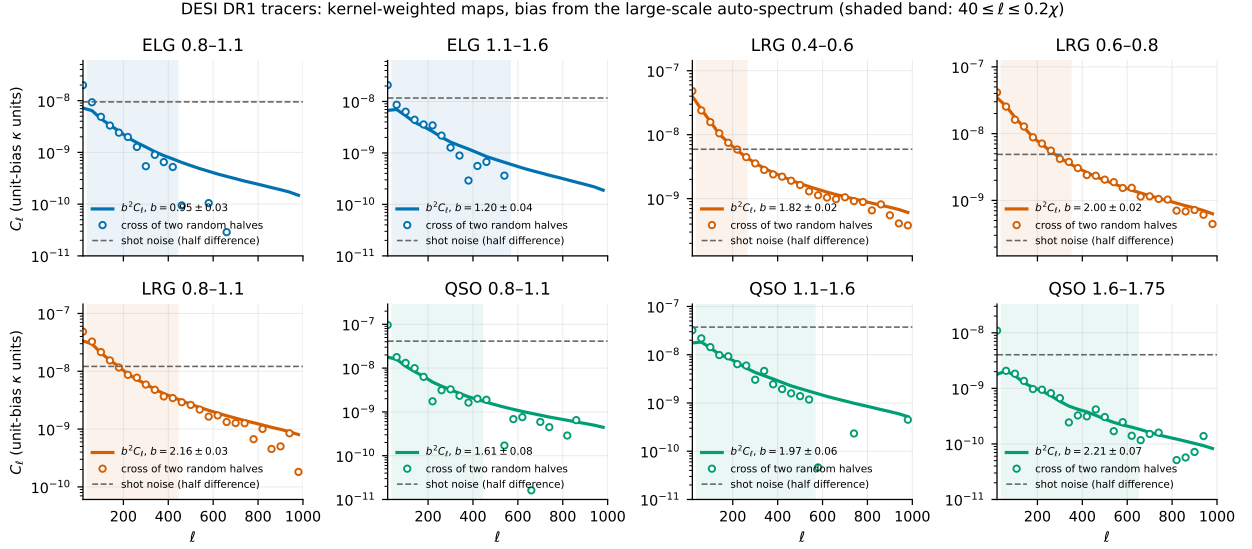
Figure 4: Angular power spectra of the eight DR1 tracer maps in convergence units for unit bias: the cross-spectrum of two random halves (points, no shot noise), the fitted b^2 C_{\ell} (line) and the shot noise measured from the half difference (dashed). The shaded band is the fit range 40 \leq \ell \leq 0.2\chi(z_{\text{mid}}) .
