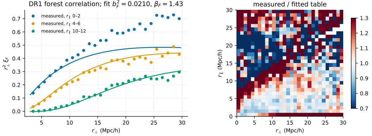
Figure 2: DR1 forest correlation from 1.8 \times 10^8 pixels: measured r_{\perp}^2 \xi_F in three radial-separation strips (points) and the fitted two-parameter table (lines); right, the ratio of the measured 1 h^{-1} Mpc cells to the fitted table (the diagonal band is the zero crossing of the anisotropic model). The fit is driven by the small separations that carry the lensing information; at r_{\parallel} < 2 and r_{\perp} > 15 h^{-1} Mpc the data exceed the model by 20–40 per cent (Section 6).
