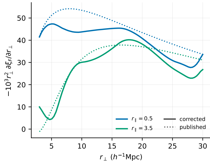
response kernel (amplitude \times 1.100 )
