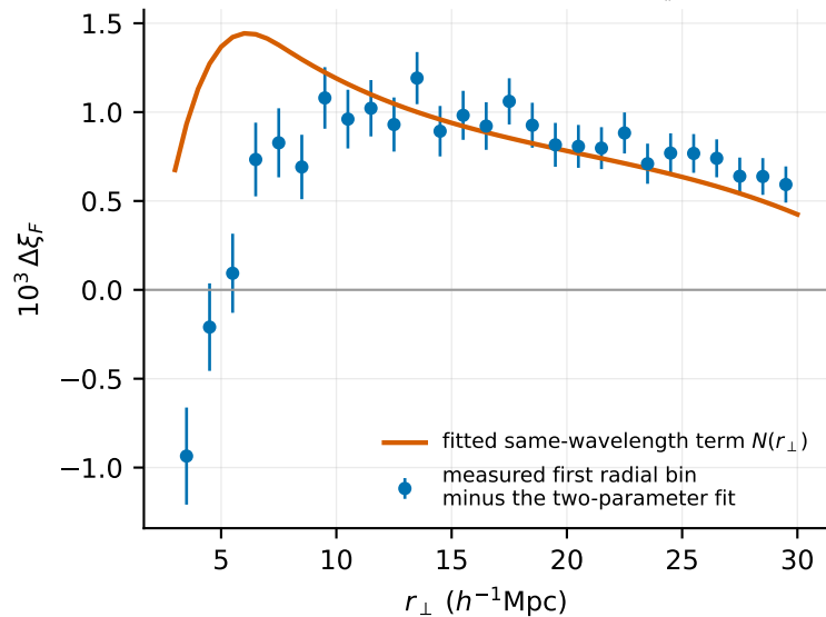
same-wavelength excess ( r_{\parallel} < 1 )
