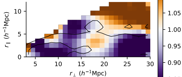
kernel ratio \xi'_{\text{new}}/\xi'_{\text{published}}
