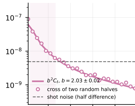
BOSS 0.4-0.6
