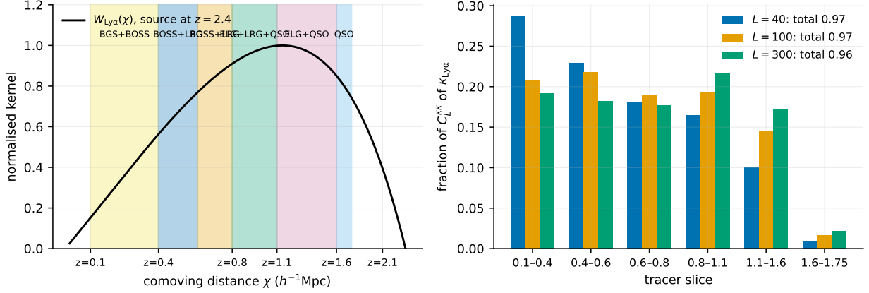
Figure 1: Left: the lensing kernel of a source at z = 2.4 (the effective forest redshift) with the six tracer slices shaded and their tracers named. Right: the fraction of the power of \kappa_{\text{Ly}\alpha} contributed by each slice at L = 40, 100 and 300 (Limber, non-linear matter power); the six slices together hold 96–97 per cent, the lowest slice alone 19–29 per cent.
