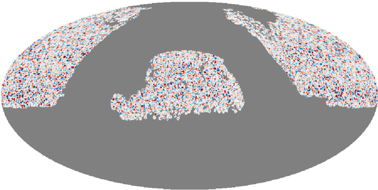
\hat{K}_{Ly\alpha} , Wiener-filtered, 40 \leq \ell \leq 400 , 30 arcmin smoothing; colour scale \pm the 99th percentile
