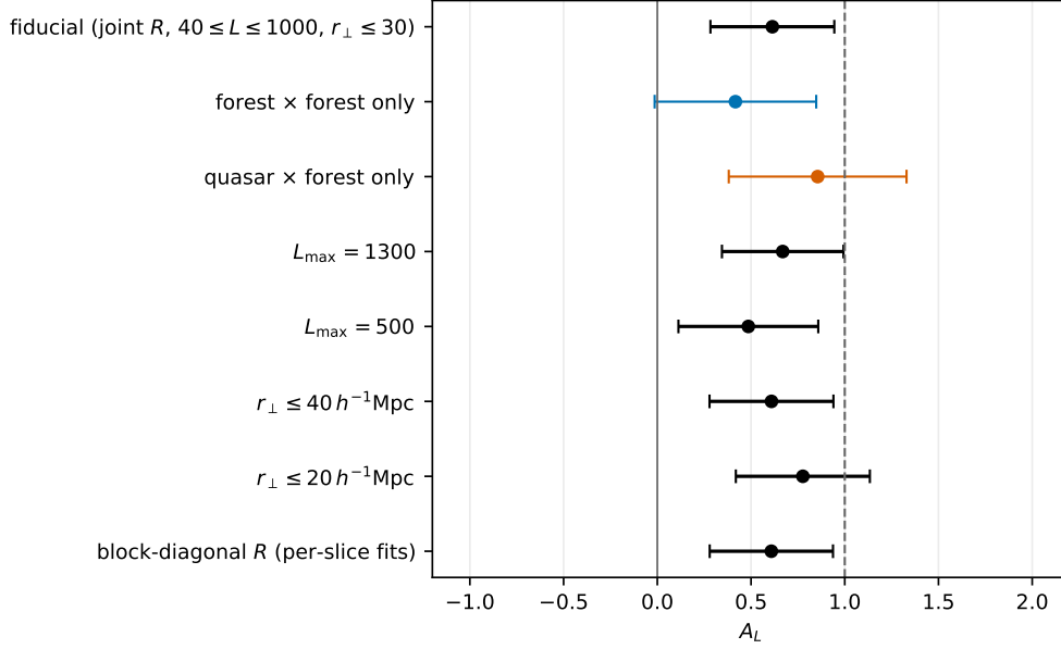
Figure 14: The lensing amplitude under the analysis variants of the paper: the fiducial combination, its two statistics, the science window widened to L = 1300 or narrowed to L = 500 , the transverse pair range widened to 40 h^{-1}\text{Mpc} or narrowed to 20 h^{-1}\text{Mpc} , and the response matrix restricted to its per-slice blocks. Jackknife errors; the lines mark A = 0 and A = 1 .
