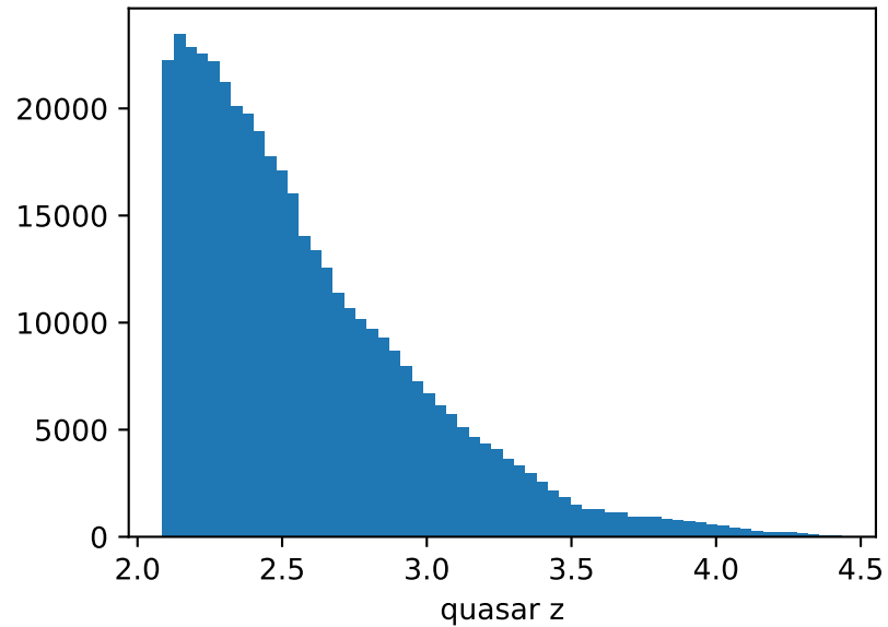
428403 forests, \sim 11043 \text{ deg}^2
