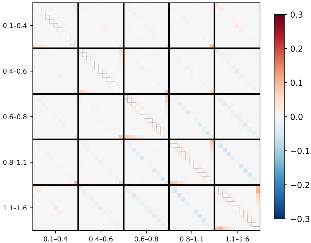
forest x forest: F_{ij}/\sqrt{F_{ii}F_{jj}} (55 components; diagonal masked)
