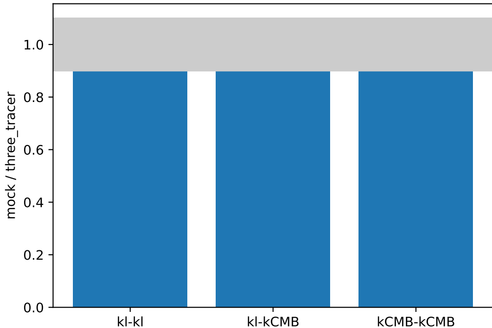
Patch spectra, 40 < L < 300
