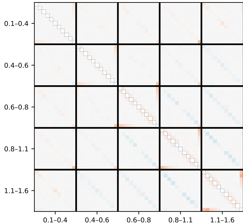
forest x forest: F_{ij}/\sqrt{F_{ii}F_{jj}} (55 components; diagonal masked)
