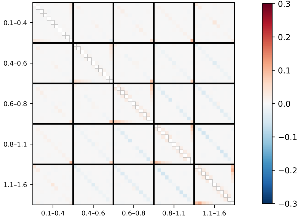
quasar x forest: F_{ij}/\sqrt{F_{ii}F_{jj}} (55 components; diagonal masked)
