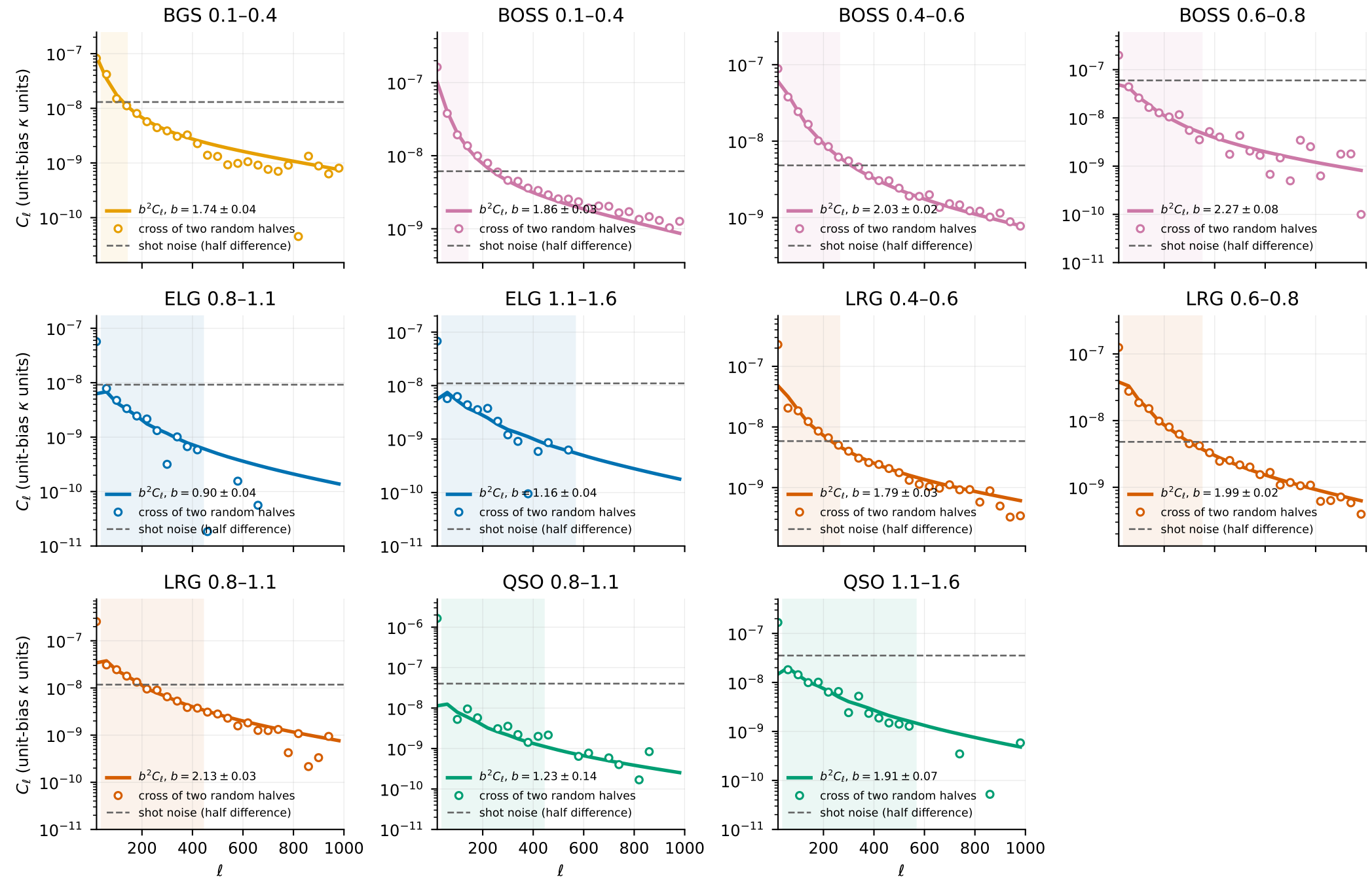
DESI DR1 and BOSS DR12 tracers: kernel-weighted maps, bias from the large-scale auto-spectrum (shaded band: 40 \leq \ell \leq 0.2\chi )
