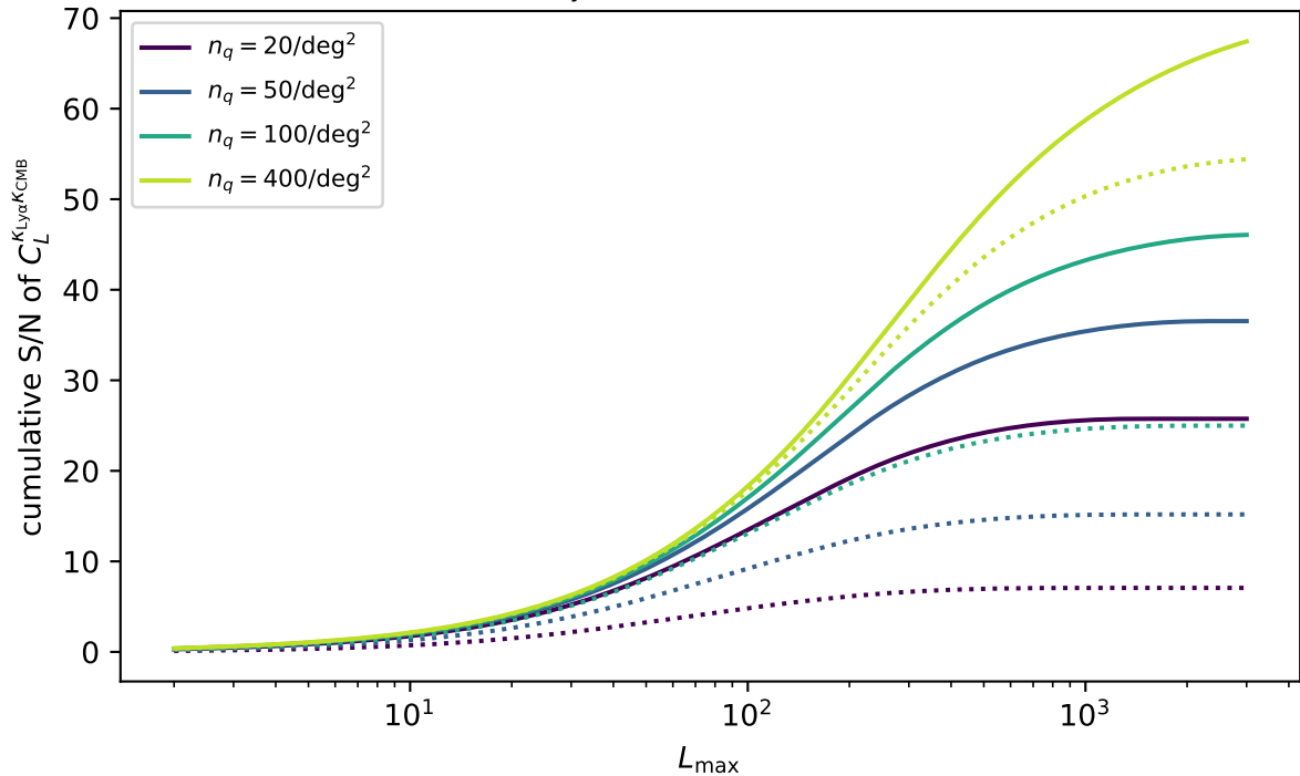
ACT-DR6-like \kappa_{\text{CMB}} , f_{\text{sky}} = 0.15 ; dotted: amplitude-hardened
